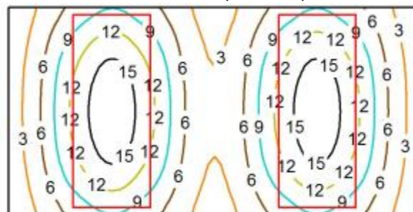
FWHM - 80° (reflector)
