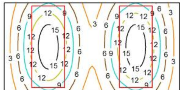
FWHM - 80° (reflector)
